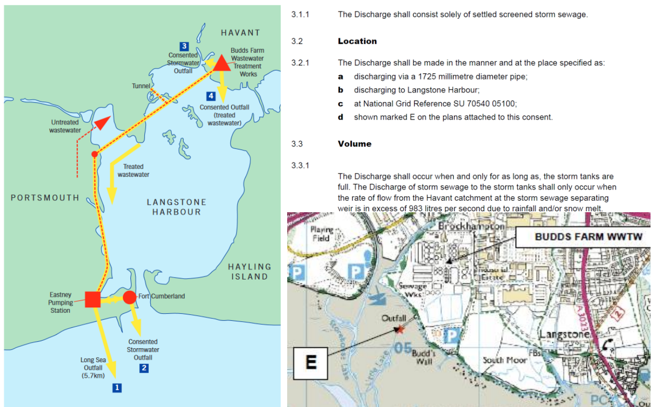
Figure 1: location of discharge outlets at Budd's Farm STW plus an extract of the EA permit for settled storm discharges into Langstone Harbour
